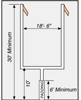
GOAL POST DETAIL
