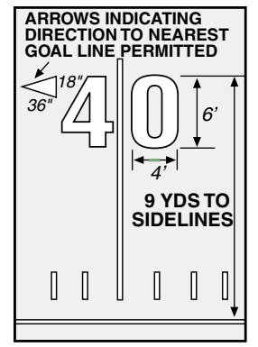
RECOMMENDED YARD-LINE NUMBERING
