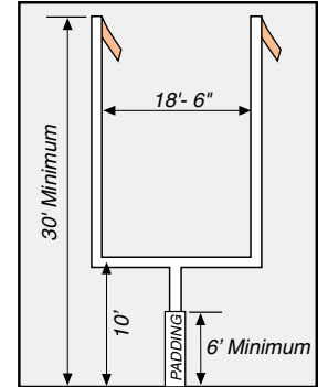
GOAL POST DETAIL
