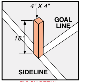
PYLON DETAIL
