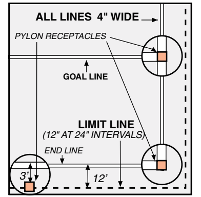
END ZONE DETAIL
