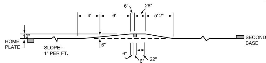
CROSS SECTION OF PITCHER'S MOUND
